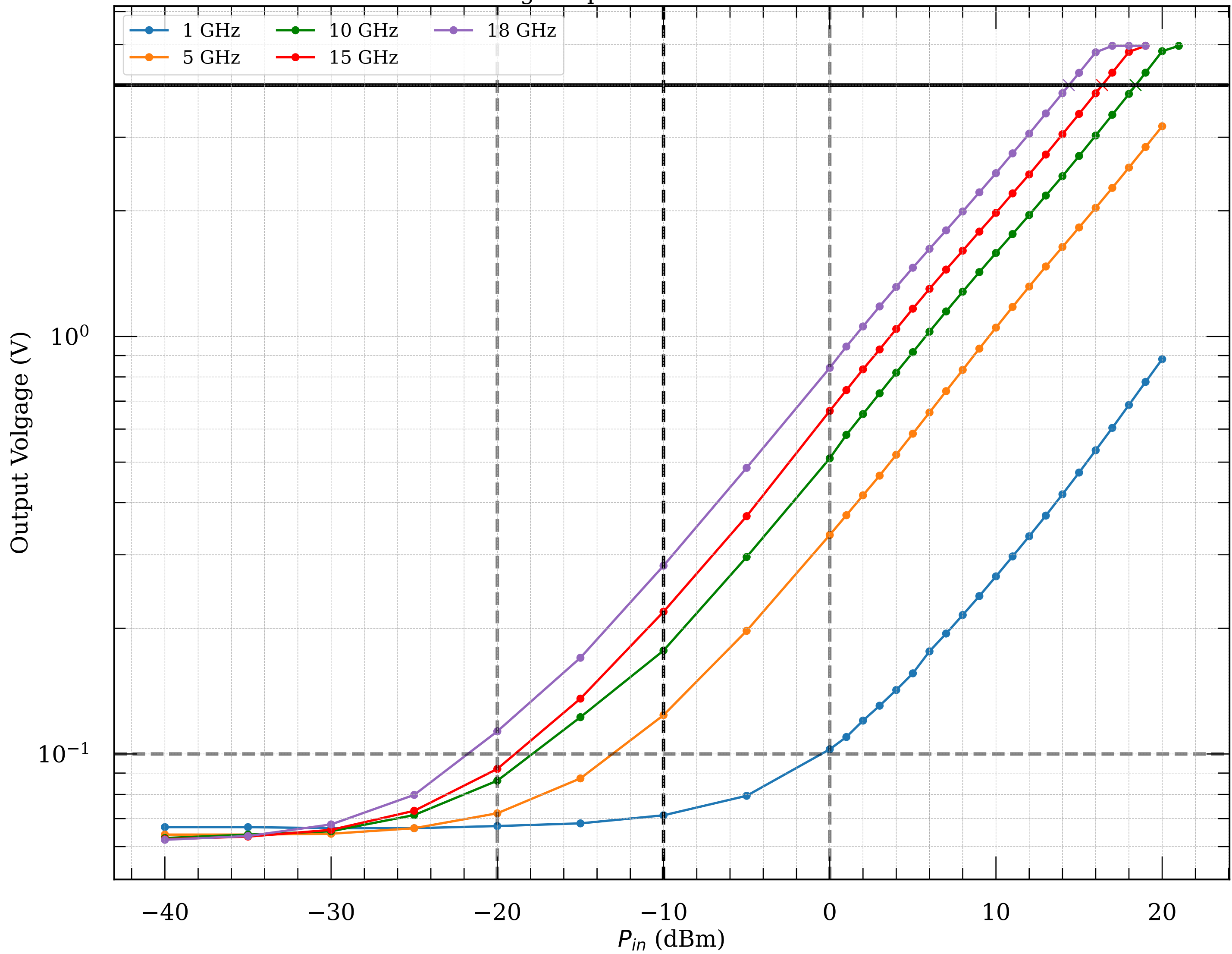
Measured voltage-to-power curve of detector module021
